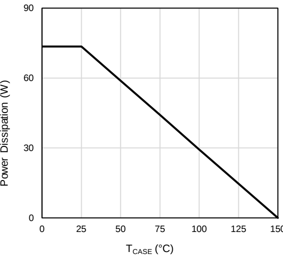
Figure 11: Power De-rating
