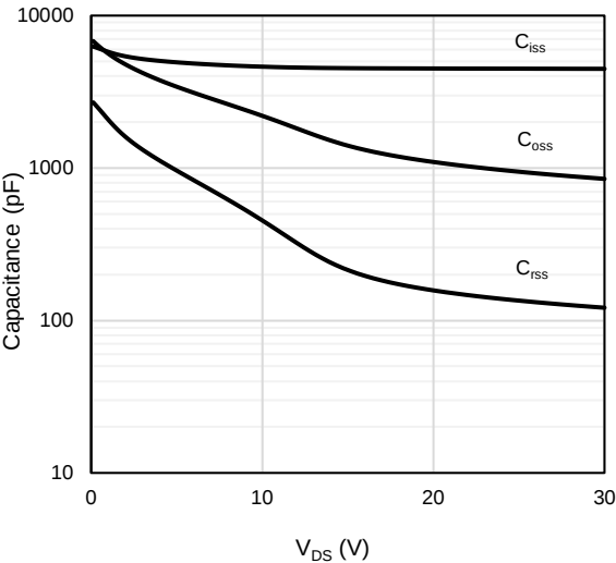
Figure 9: Capacitance Characteristics
