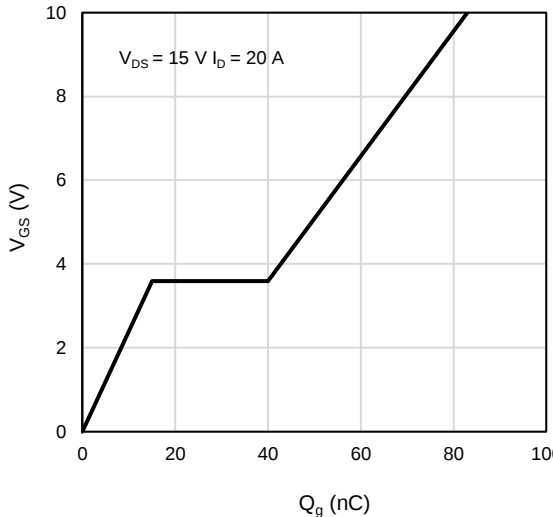
Figure 10: Gate-Charge Characteristics
