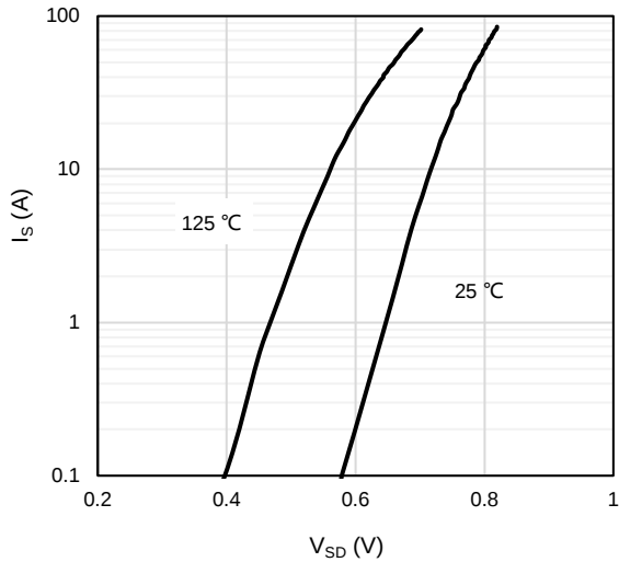
Figure 7: Body-Diode Characteristics
